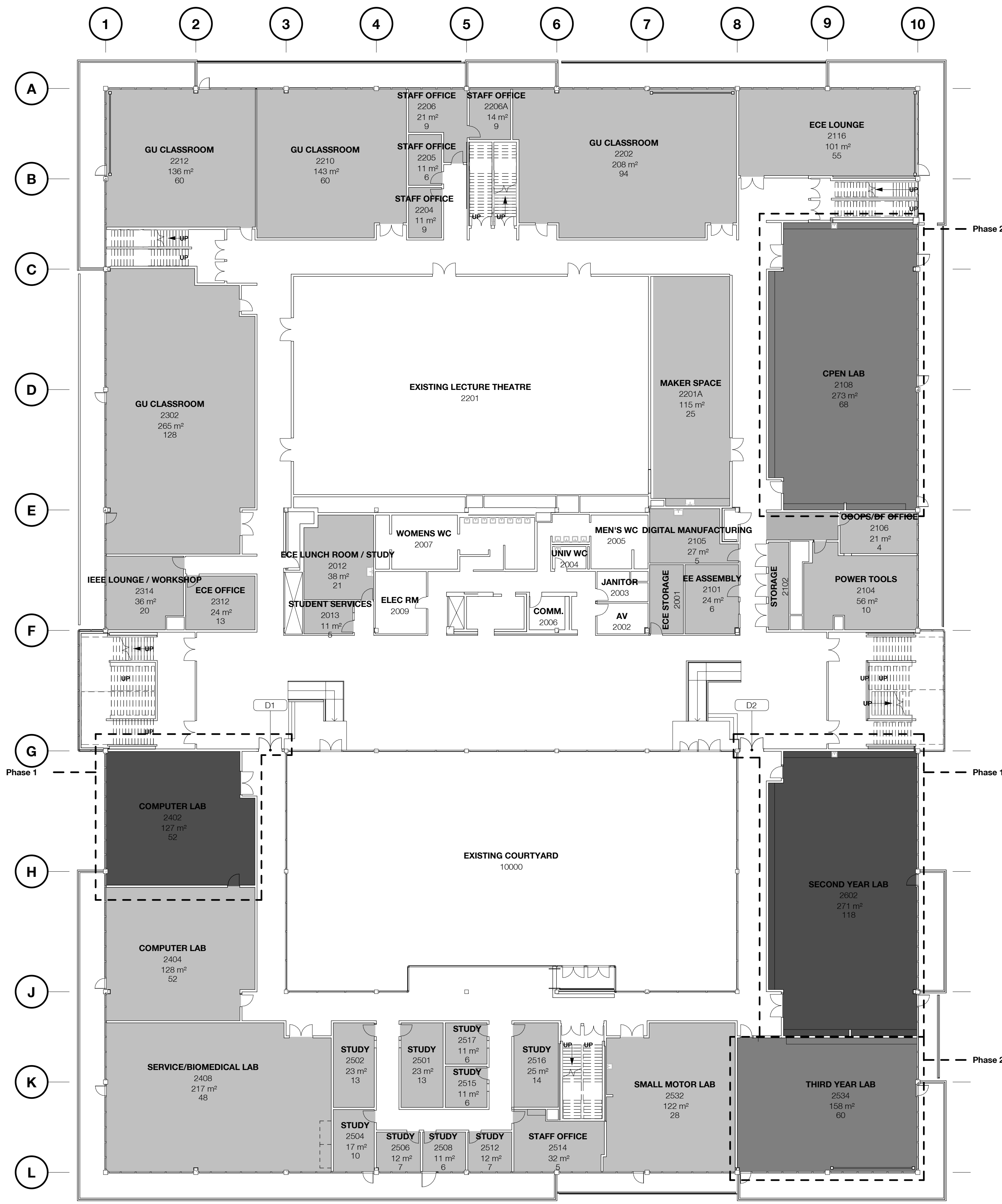
1 Level 02 Phasing and Scope Plan A0.05 1 : 200
